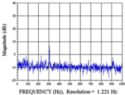
Figure 5. Spectral Analysis ~ Healthy / low level, no significant peaks with harmonics.
